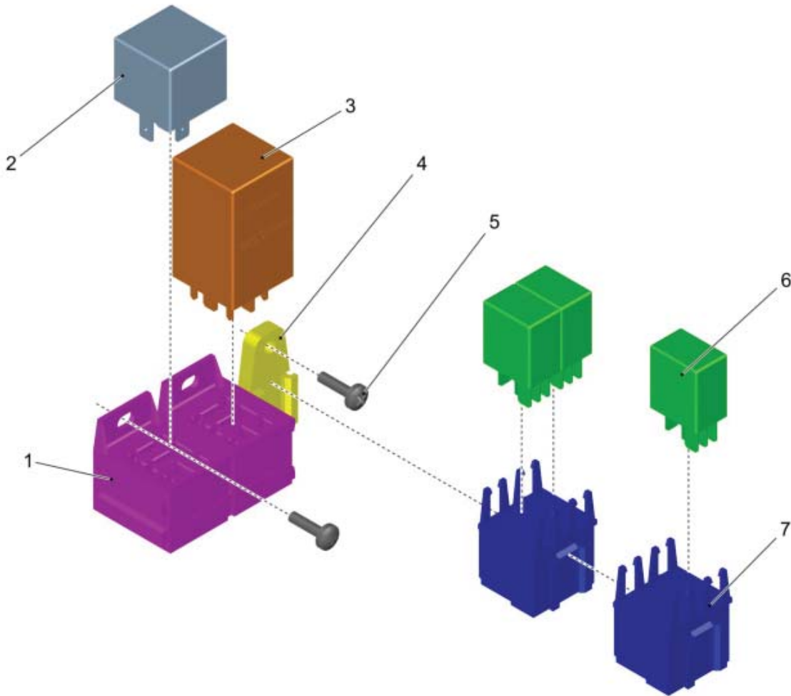
PARTS LIST - SIDE CONSOLE R.H.
